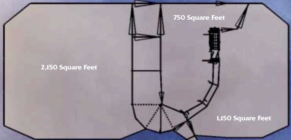
Classic 350-210 System
